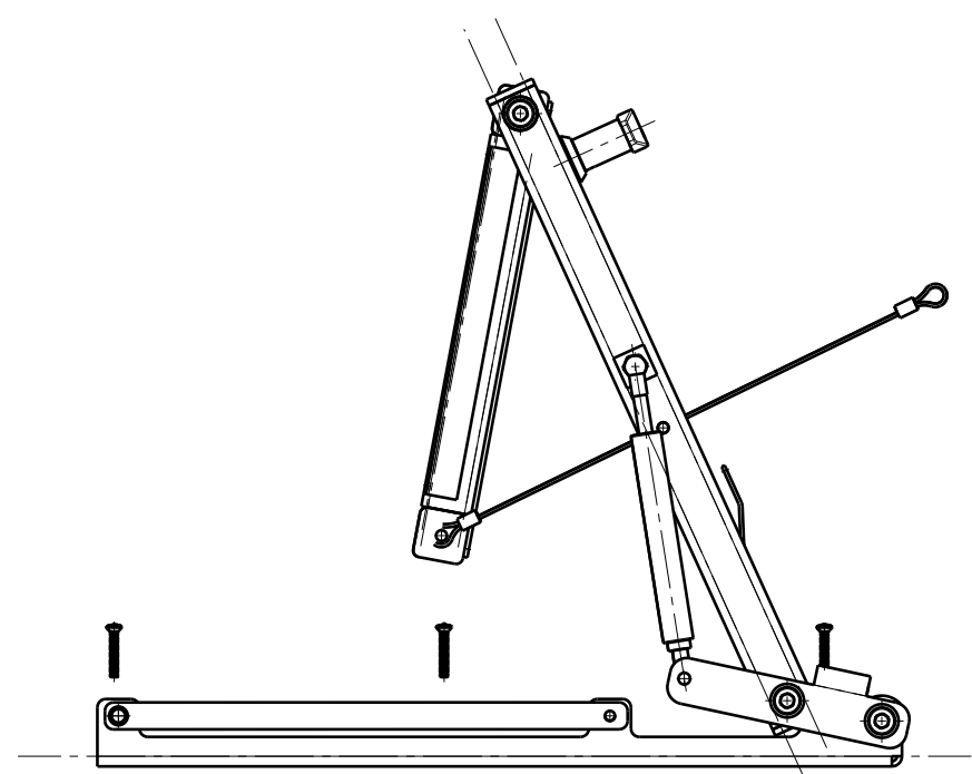
Auxiliary view A Scale: 1:5
