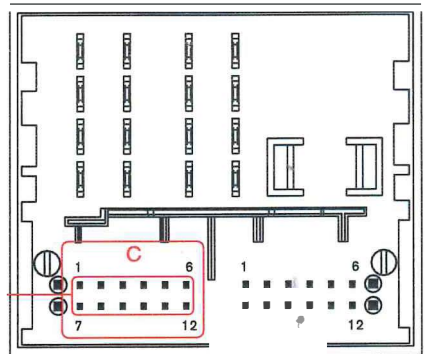
FIG 1.2 Quadlock Connector (Rear of monitor)
